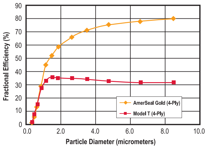
4-Ply Ring Panel Filter Composite Minimum Efficiency Curve Per ASHRAE 52.2
