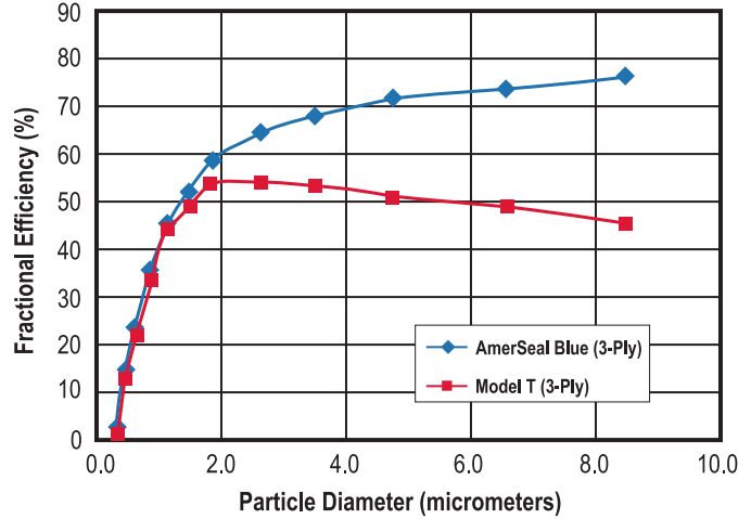
3-Ply Ring Panel Filter Composite Minimum Efficiency Curve Per ASHRAE 52.2
