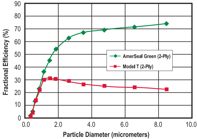
2-Ply Ring Panel Filter Composite Minimum Efficiency Curve Per ASHRAE 52.2
