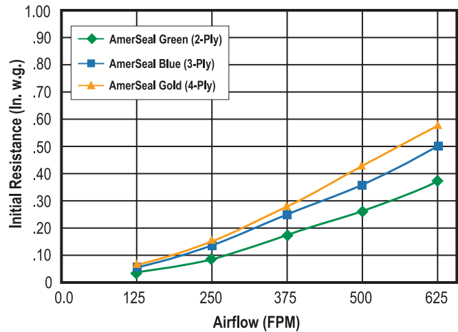
Filter Initial Resistance vs. Airflow
